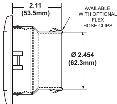
4" SANTA FE LOUVER W/ 2-1/2" HOSE ADAPTER
