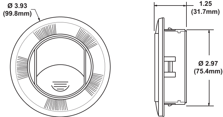
4" SANTA FE LOUVER W/O HOSE ADAPTER
