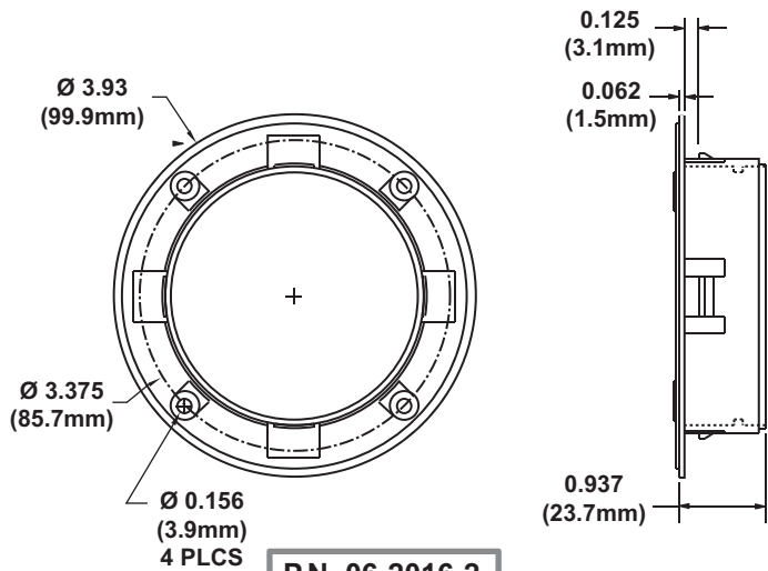
4" TRADITIONAL MOUNTING RETAINER
