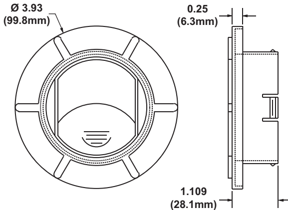
4" TRADITIONAL FRONT PANEL W/ VANES
