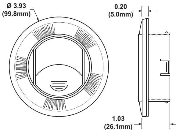
4" SANTA FE FRONT PANEL W/ VANES
