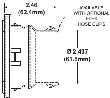
4" TRADITIONAL LOUVER W/ 2-1/2" HOSE ADAPTER
