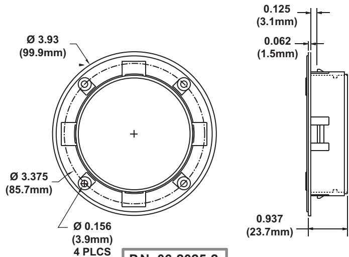
4" SANTA FE MOUNTING RETAINER
