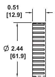
STARLIGHT MOUNTING BEZEL
