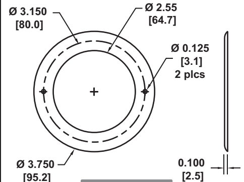
MOUNTING BEZEL
