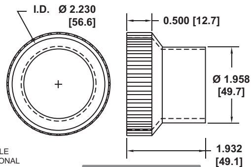
MOUNTING BEZEL
