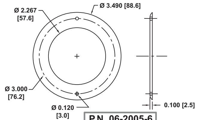
MOUNTING BEZEL
