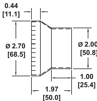
CANYON BALL & RETAINER
