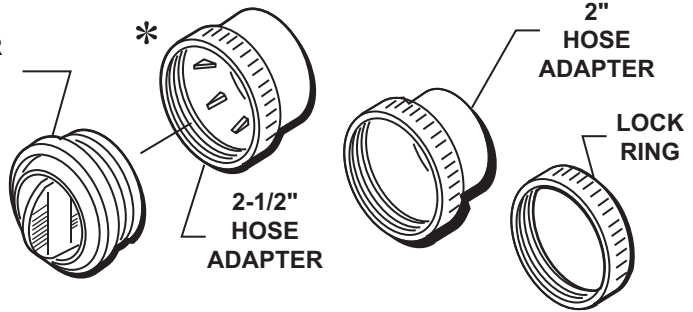
2-1/2" CANYON LOUVER (BALL / RETAINER)
