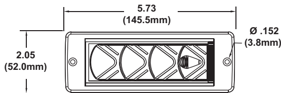
NARROW FRAME VERSION WITH HOLES P.N. 06-2020-2
