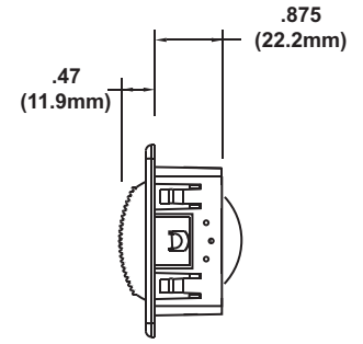
WITHOUT HOSE ADAPTER
